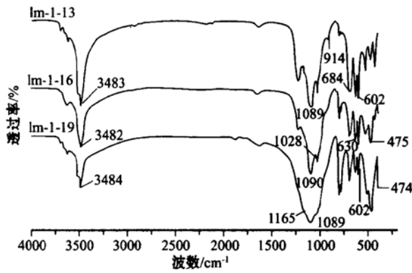
图 2 昌化鸡血石中明矾石的红外光谱图 Fig. 2 IR patterns of alunite in Changhua Chicken_Blood Stone
