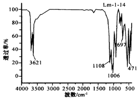
图 3 昌化鸡血石中迪开石的红外光谱图 Fig. 3 IR patterns of dickite in Changhua Chicken_Blood Stone
