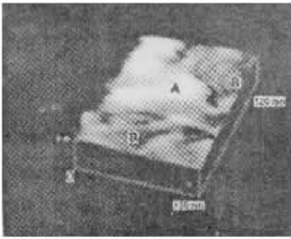
图9b 辉锑锡铅矿{100}解理面的STM微形貌图 Fig.9b STM microtopographic image of the {100} cleavage surface of franckeite V_b=10.0\text{mV} , I_{\text{ref}}=1.08\text{nA} 扫描范围: 125nm×125nm
